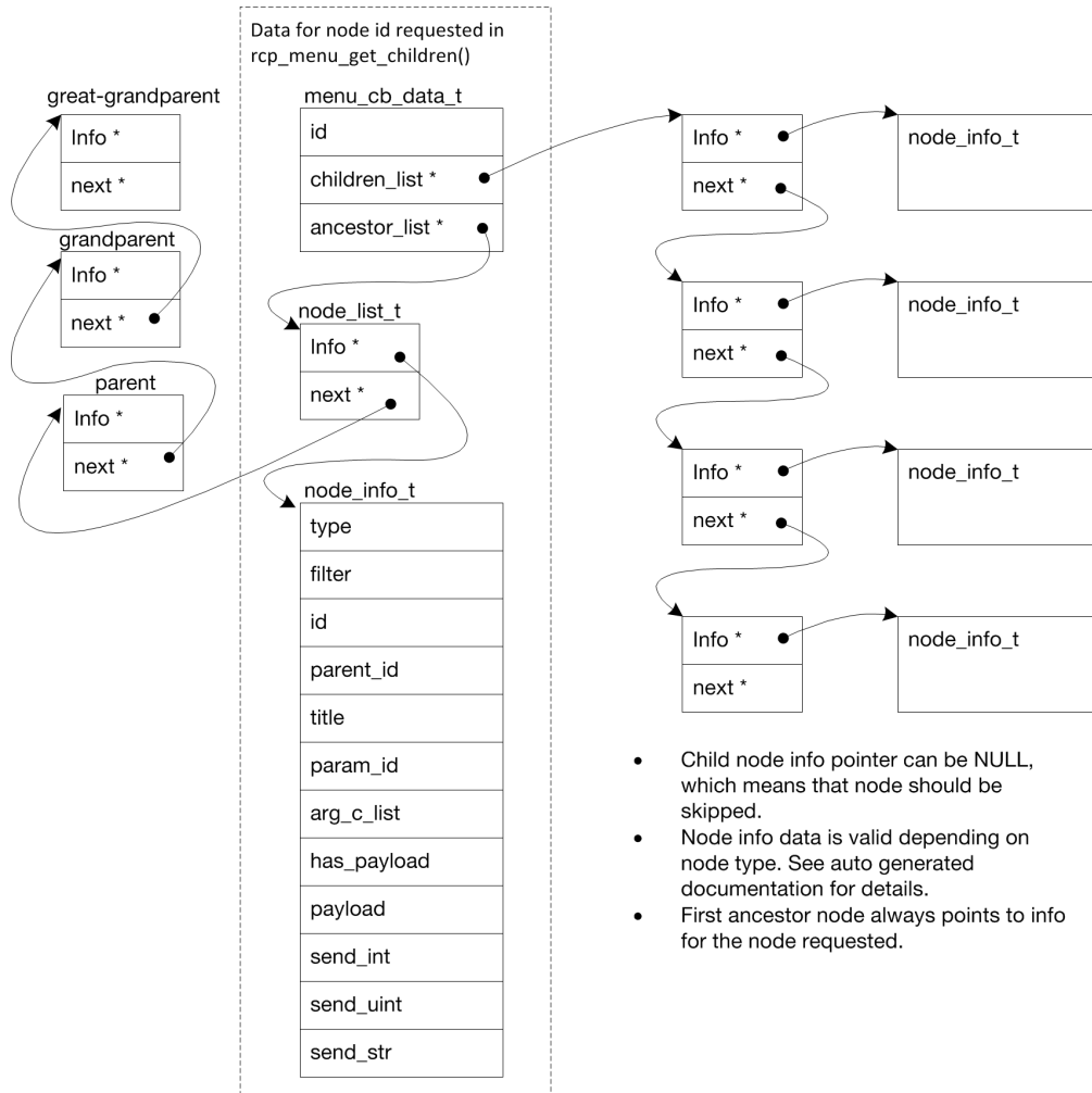
Figure 8. Menu Tree Data Structures
