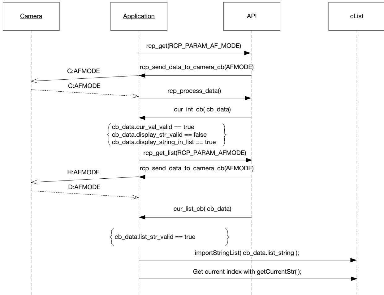
Figure 6. Getting Display String from List
