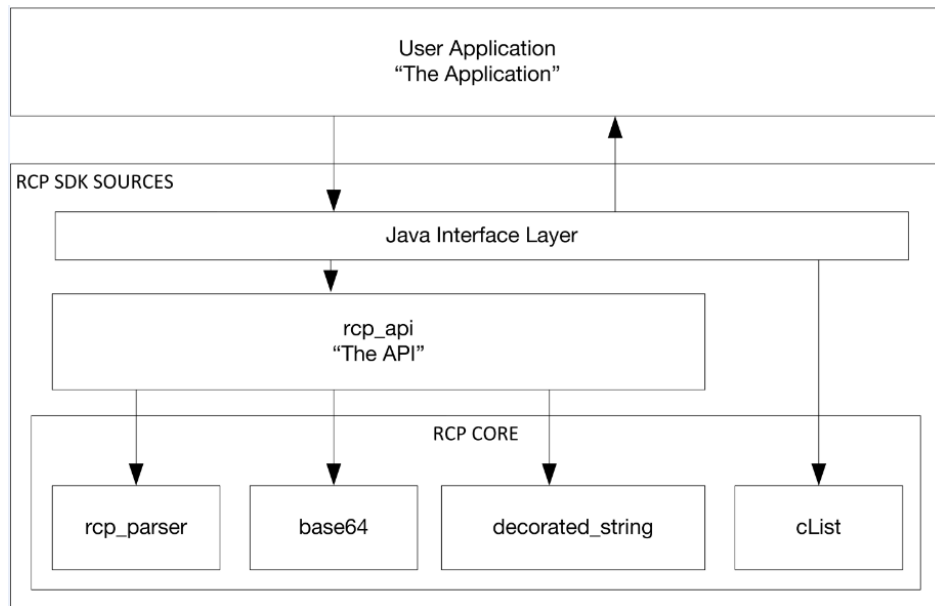
Figure 2. SDK and Application Relationship for Java
