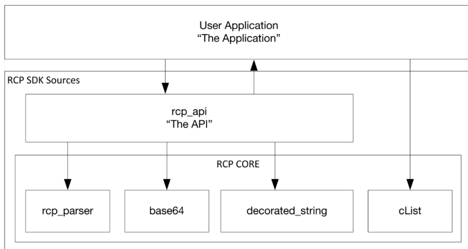
Figure 1. SDK and Application Relationship for C and C++
