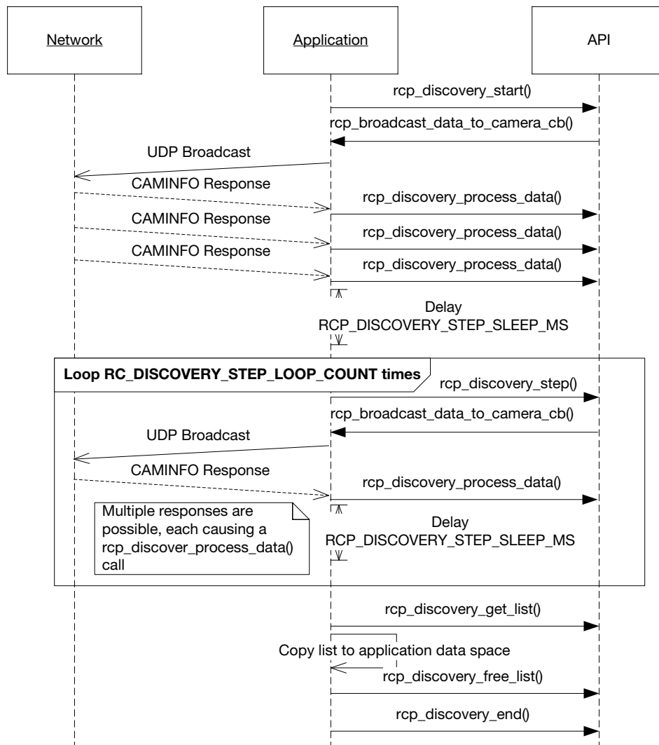
Figure 3. Discovery Process Sequence
