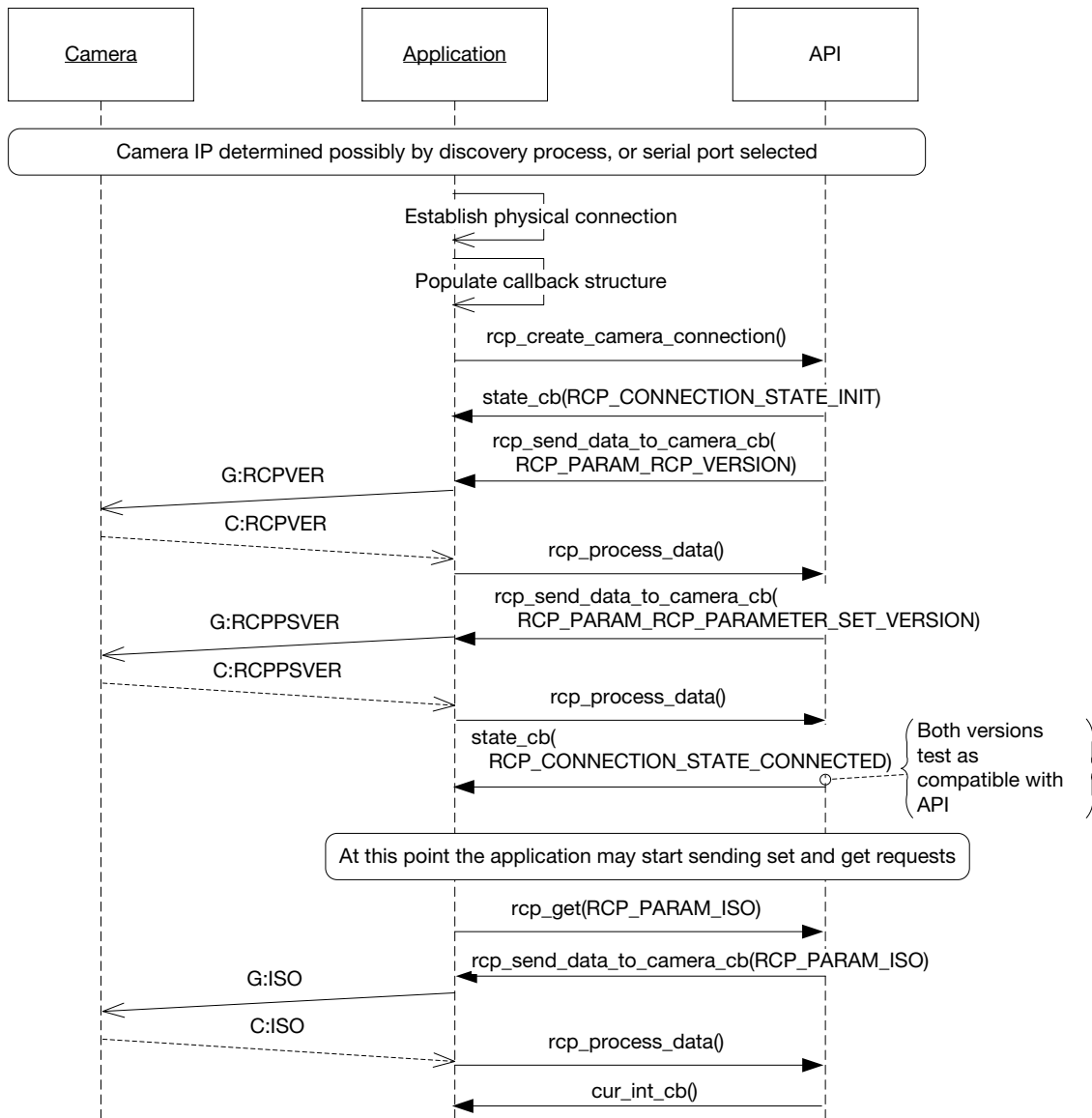
Figure 4. Camera Connection Sequence
