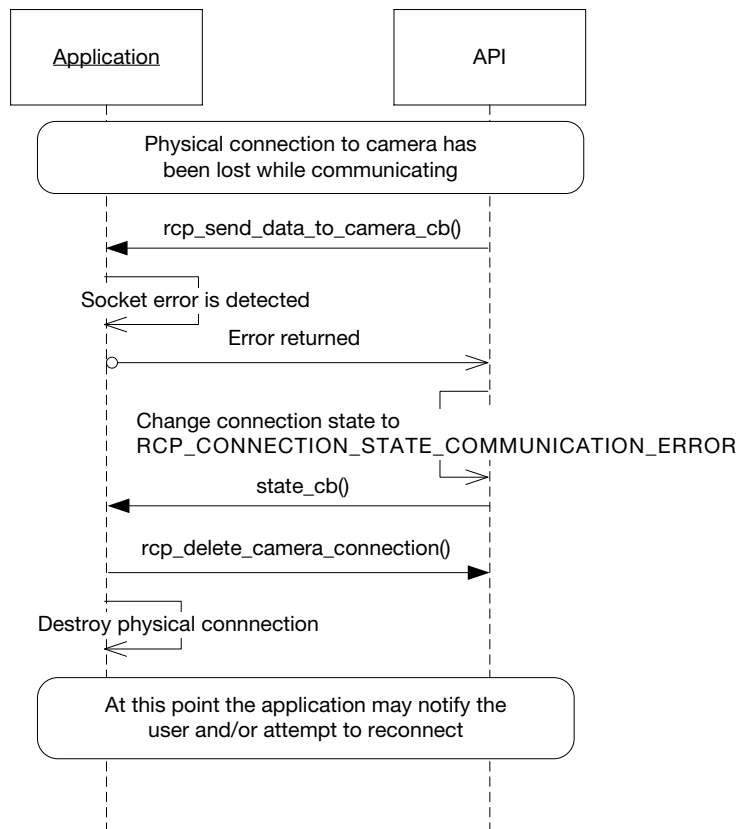
Figure 5. Correct Connection Error Recovery Sequence
